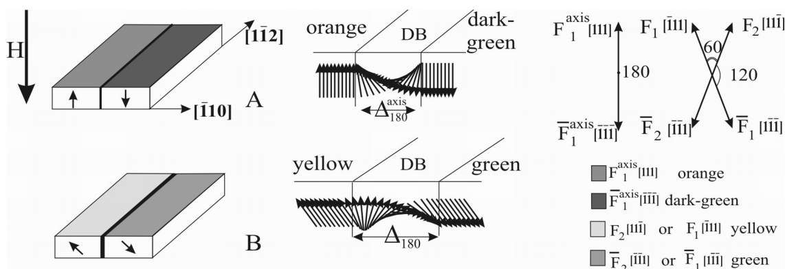
Fig. 3. Models of domain structures and magnetization distribution in domain wall: a — 180° axial; b — 180° angular.
